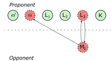
Fig. 21. The update made to the Argument Interchange Format structure and the argumentation framework upon Proponent's creation of the revised proof (1-n).
