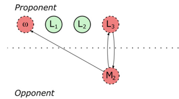
Fig. 19. The update made to the Argument Interchange Format structure (on the left-hand side) and the argumentation framework (on the right-hand side) upon Opponent's counter of L_3 (1-l).
