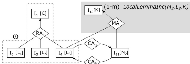
Fig. 20. The update made to the Argument Interchange Format structure and the argumentation framework upon Proponent's introduction of a new lemma, K , replacing L_3 (1-m).
