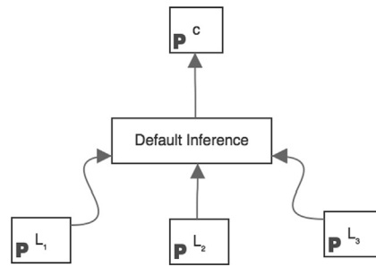
Fig. 4. Lemmas, conjecture and proof.
